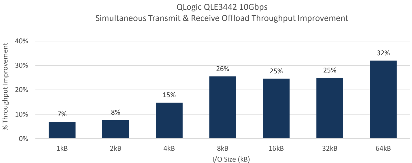
Figure 5. QLogic QLE3442 10Gbps Simultaneous Transmit and Receive Offload Throughput Improvement
