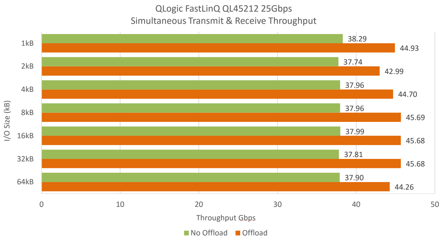
Figure 8. QLogic FastLinQ QL45212 25Gbps Simultaneous Transmit and Receive Throughput
